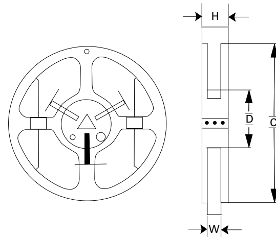
Reel Specifications
